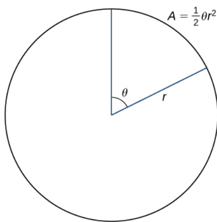
Figure 7.40 The area of a sector of a circle is given by A = \frac{1}{2} \theta r^2 .
