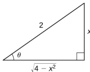
Figure 3.6 A reference triangle can be constructed for Example 3.22 .
