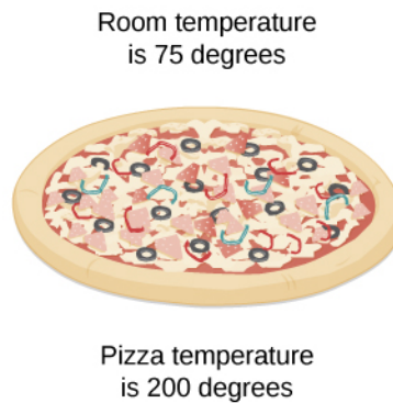
Figure 4.17 From Newton's law of cooling, if the pizza cools 10°F in 1 minute, how long before it cools to 150°F?
