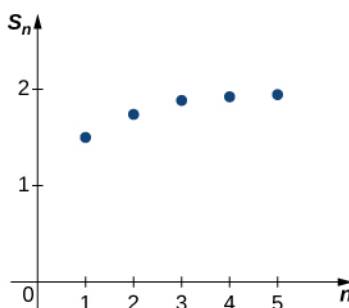
Figure 5.10 The graph shows the sequence of partial sums \{S_k\} . It appears that the sequence is approaching the value 2.
