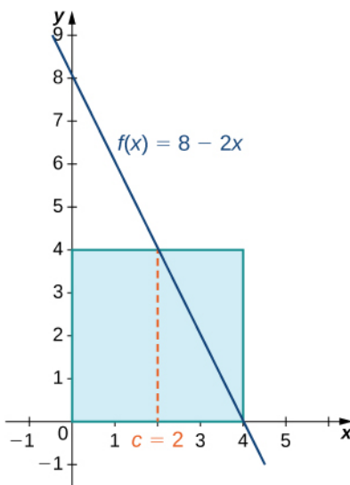
Figure 1.26 By the Mean Value Theorem, the continuous function f(x) takes on its average value at c at least once over a closed interval.
