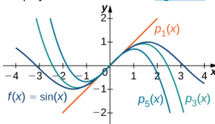
Figure 6.7 The graph shows the function y = \sin x and the Maclaurin polynomials p_1, p_3 and p_5 .
