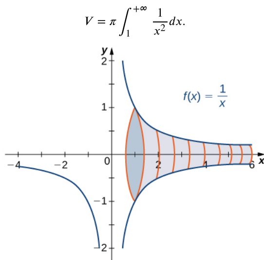
Figure 3.19 The solid of revolution can be generated by rotating an infinite area about the x -axis.
