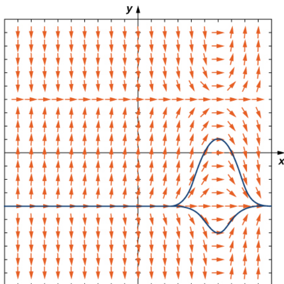
Figure 4.9 Direction field for the differential equation y' = (x - 3)(y^2 - 4) showing two solutions. These solutions are very close together, but one is barely above the equilibrium solution y = -2 and the other is barely below the same equilibrium solution.
